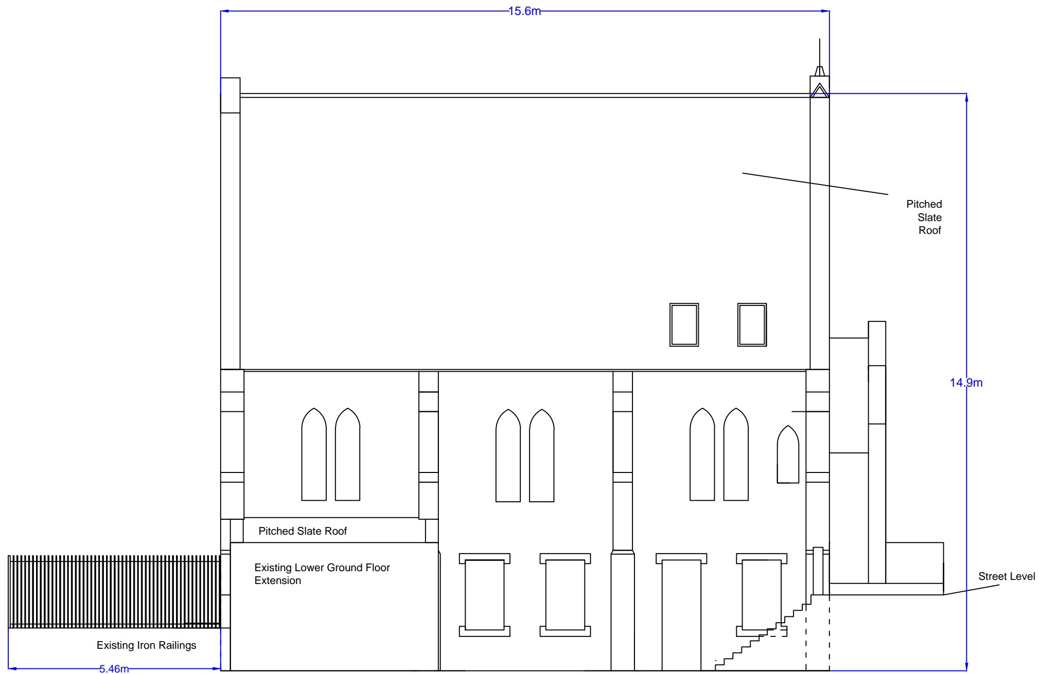
8DT8: 8 Derby Terrace West Elevation As Proposed Page 1 of 1, Scale 1:100 at A3
